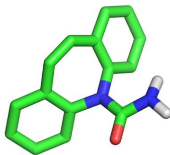
carbamazepine
